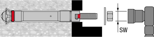
7. Attaching the belonging washer
