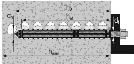
Hollow brick with threaded rod HIT-V and two sieve sleeves HIT-SC for deeper embedment depth
