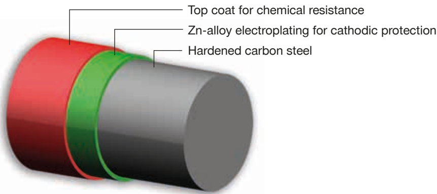
Fig. 32: Illustration of multilayer coating on fasteners and connectors.
