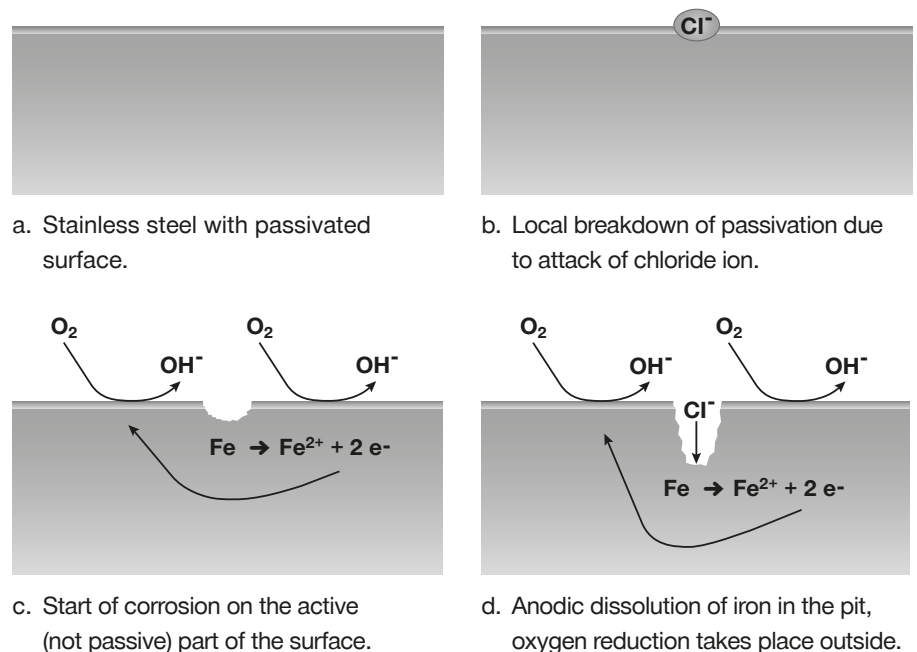
Fig. 6: Phases of pitting corrosion on stainless steel.
