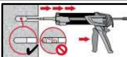
Injection method for drill hole depth
