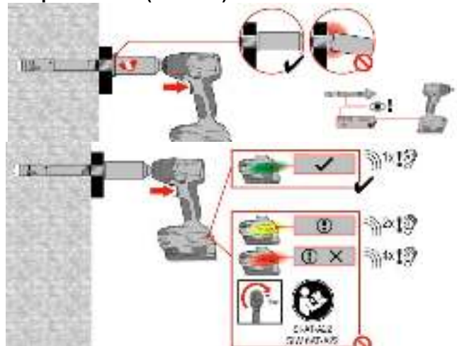
4b. Torque with impact wrench with Adaptive torque module (M8-M12)
